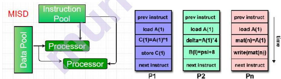
Figure 2.7 Multiple-instruction, single-data (MISD) architecture.
