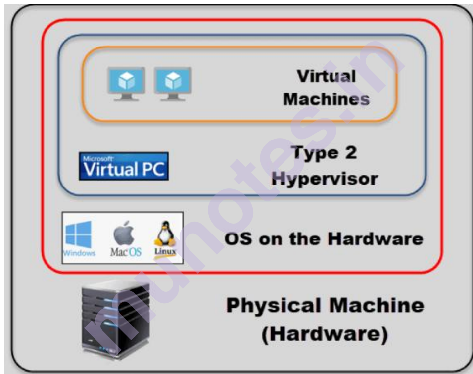
FIGURE 3.8 Type 2 Hypervisor
