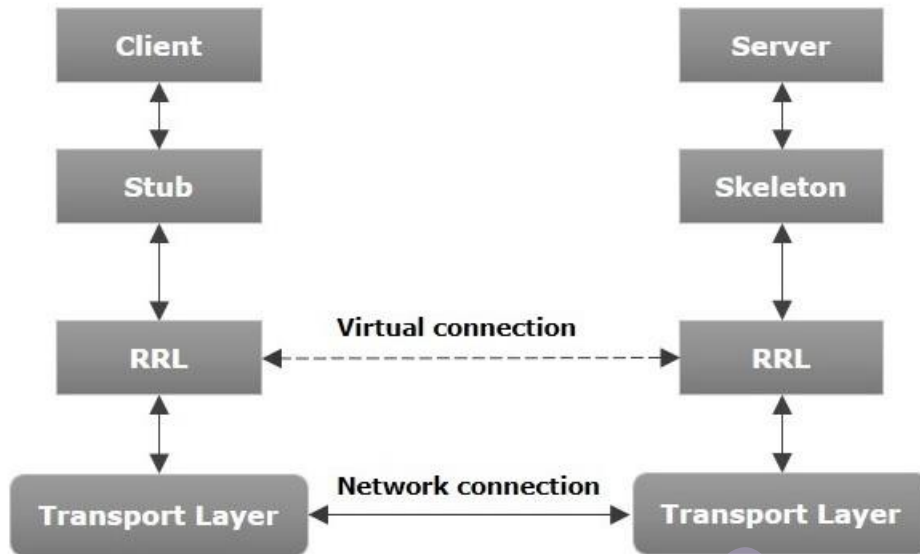
Figure 2.25 Java remote method invocation (RMI)
