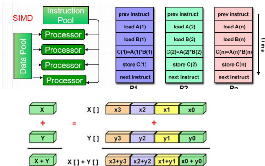
Figure 2.6 : Single-instruction, multiple-data (SIMD) architecture.
