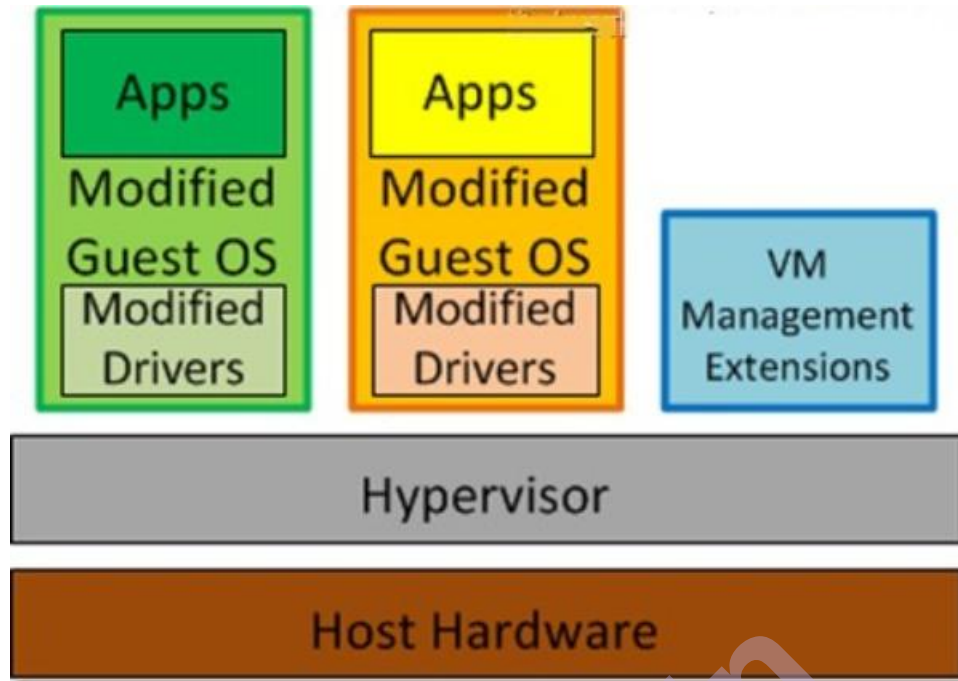
FIGURE 3.12 Paravirtualization
