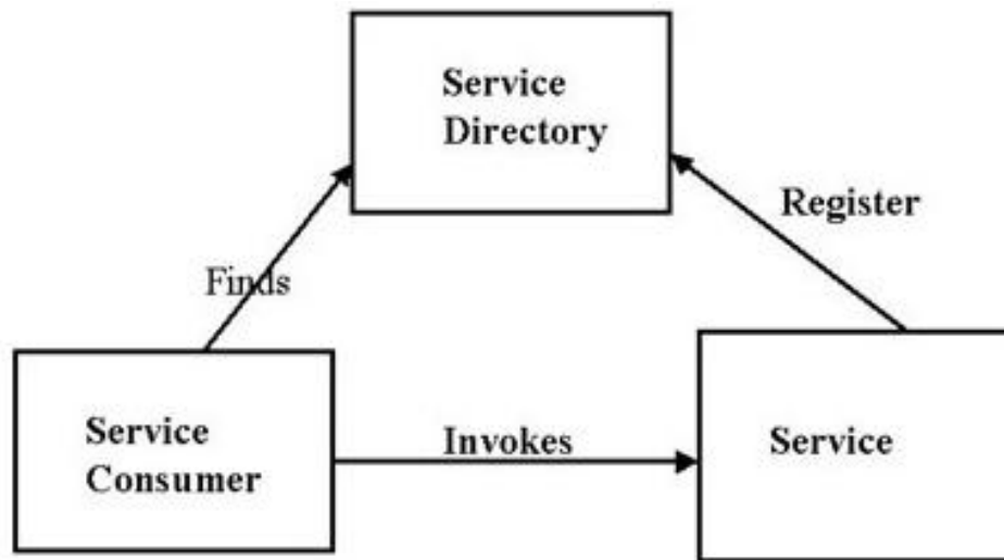
Figure 1.17 Service-oriented Architecture
