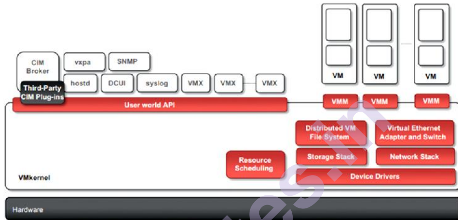
FIGURE 3.21 VMware ESXi server architecture (Reference from “Mastering Cloud Computing Foundations and Applications Programming” by Rajkumar Buyya)
