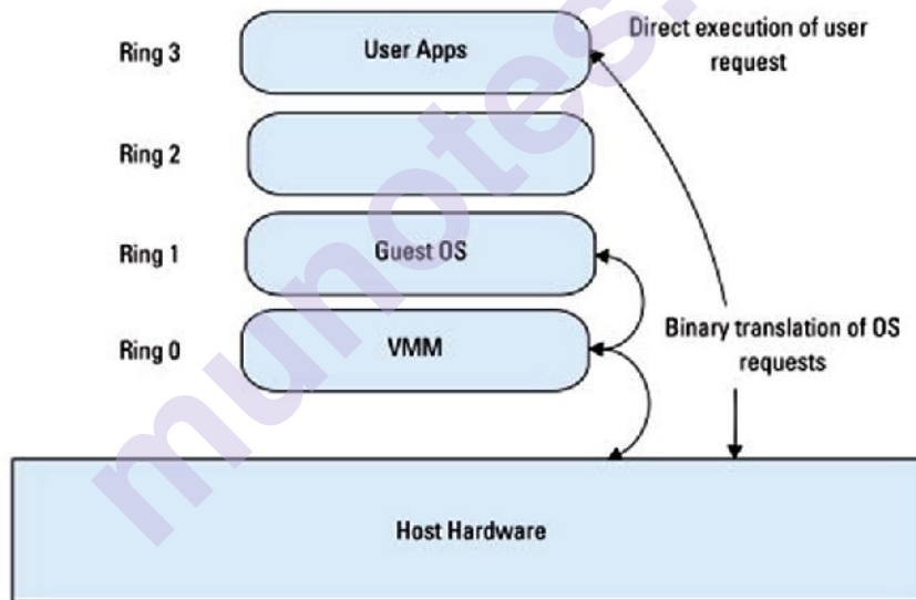
FIGURE 3.11 Full Virtualization
