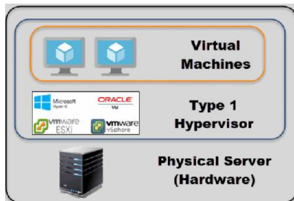
FIGURE 3.7 Type 1 Hypervisor
