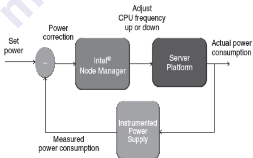
Figure 5.4 Server power management control loop
