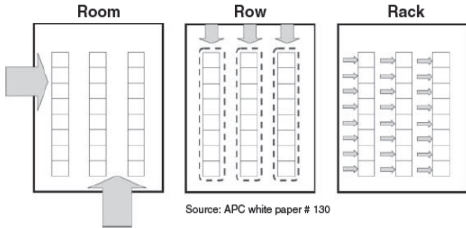
Figure 5.2 Room, row and rack level cooling
