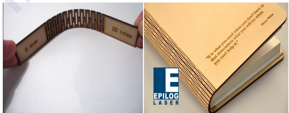
The lattice (or living) hinge.
